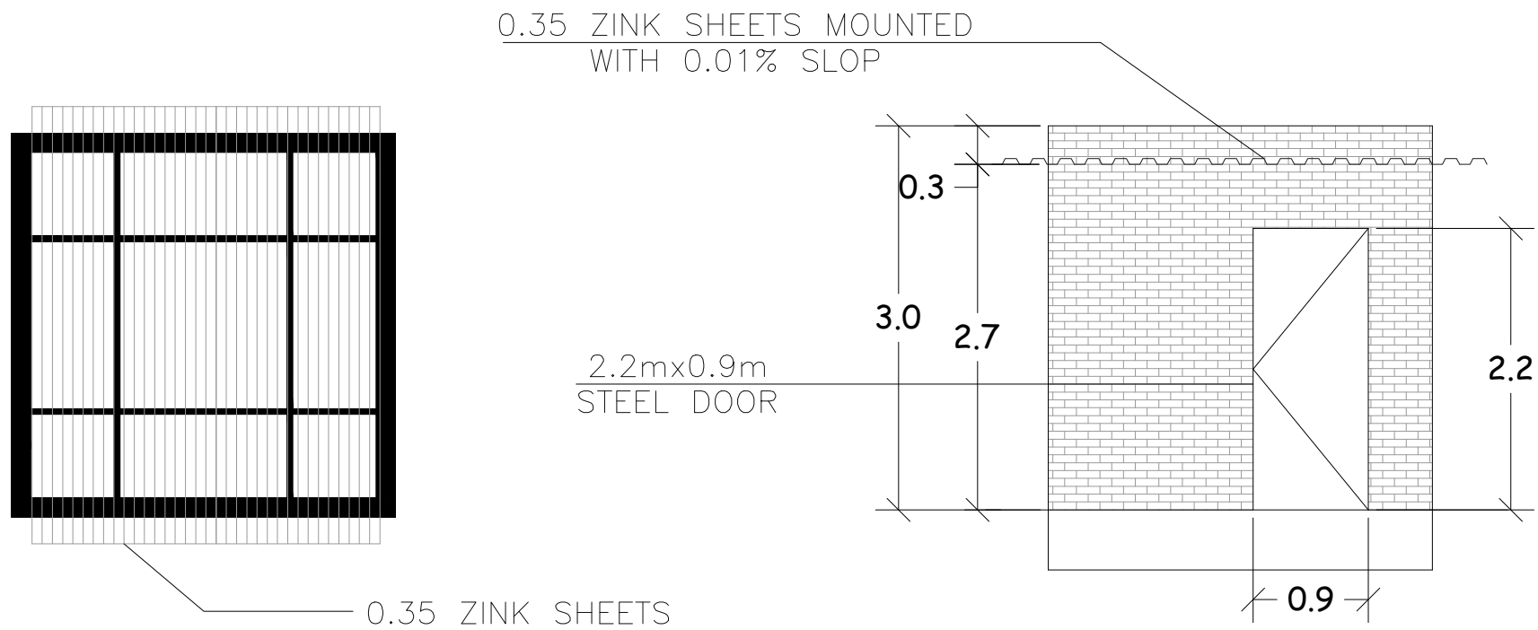
3 CONTROLLER ROOM ROOF
