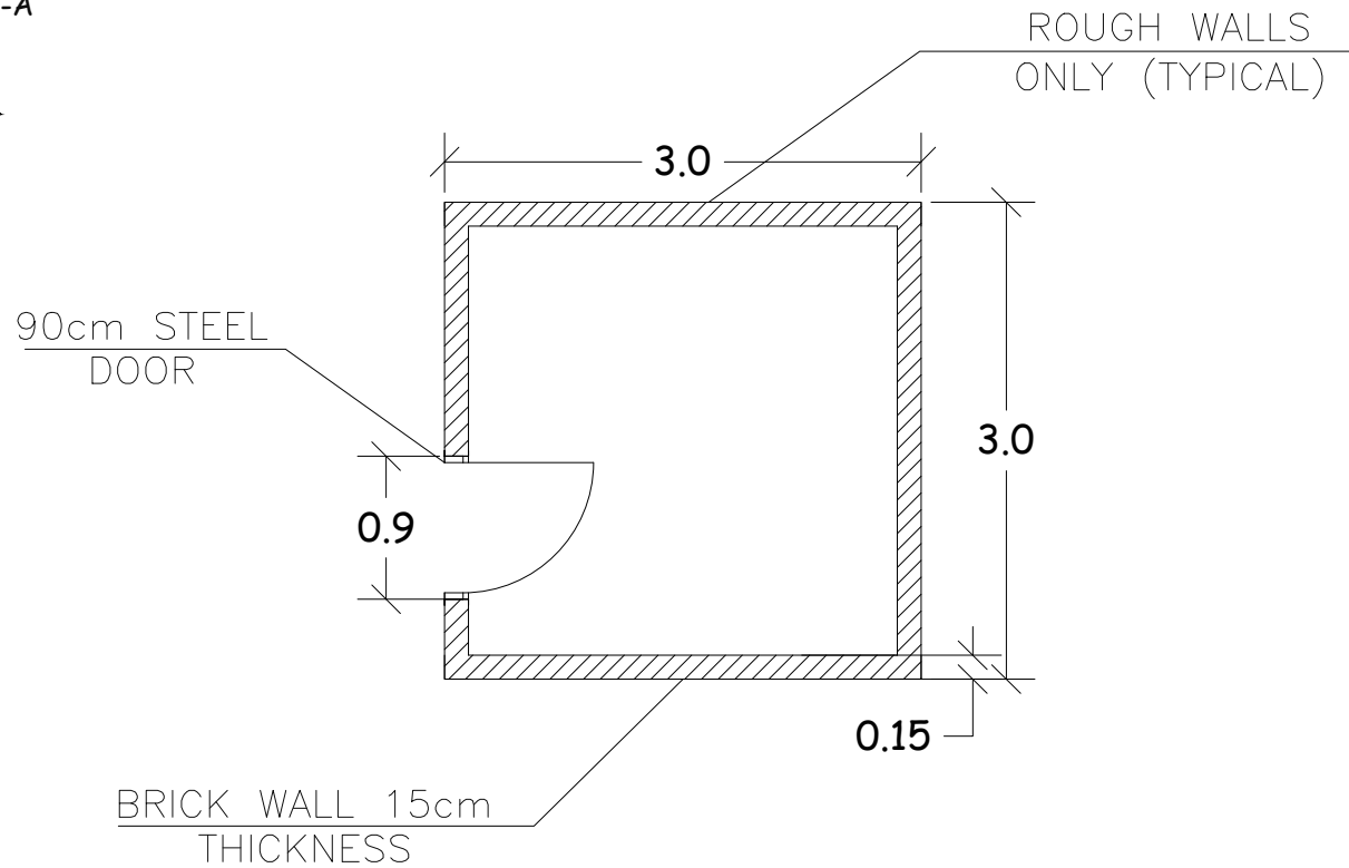
1 CONTROLLER ROOM BOUNDARIES
